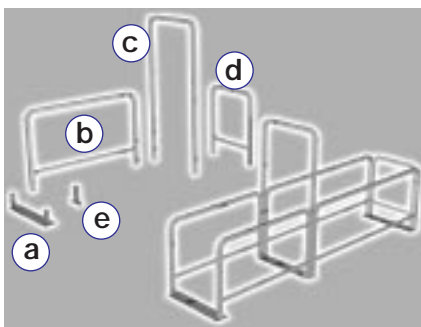
Exterior cart corral components (all components are made from 1.5" galvanized or stainless steel)
